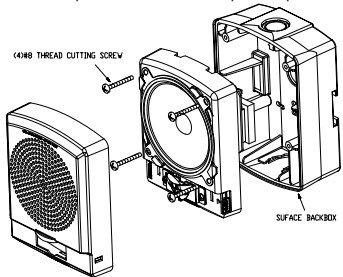
Figure 6: Surface Backbox Mounting
