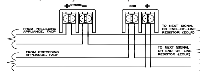
Figure 1: Strobe Wiring
