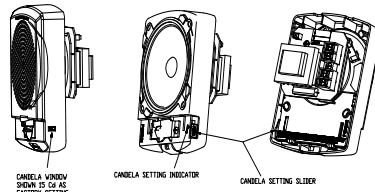
Figure 4: Strobe Candela indicator
