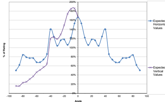
Figure 5: LSPST3 and LSPST3-A Expected Light Output
