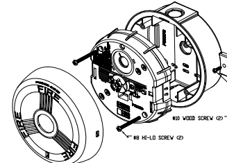
Figure 5: Ceiling Horn Strobe with LSPKBB Surface Mounting Box
