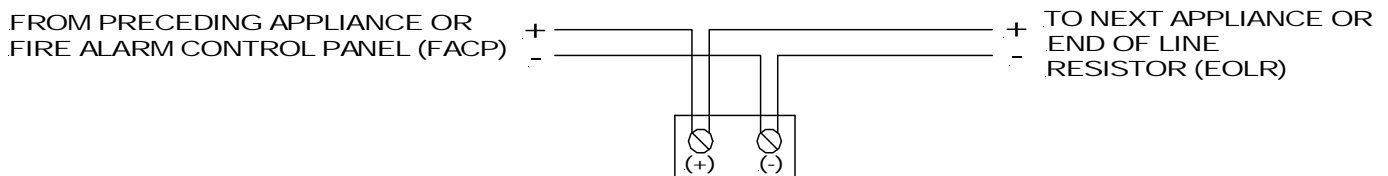
Figure 4: Wiring Diagram
