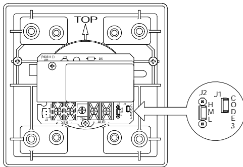
Figure 1: Showing Location of Jumper Plugs
