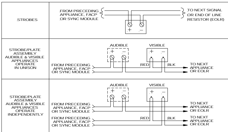
Figure 1: Wiring Diagrams
