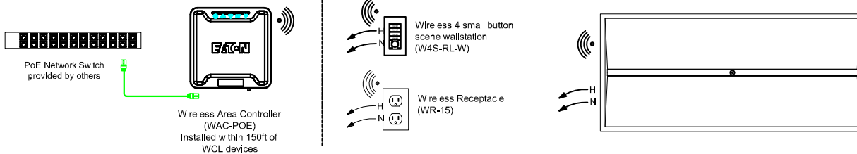
Encounter 2x4 with INstinct Sensor 24EN-LD2-34-UNV-L835-CD1-SWPD1-U
