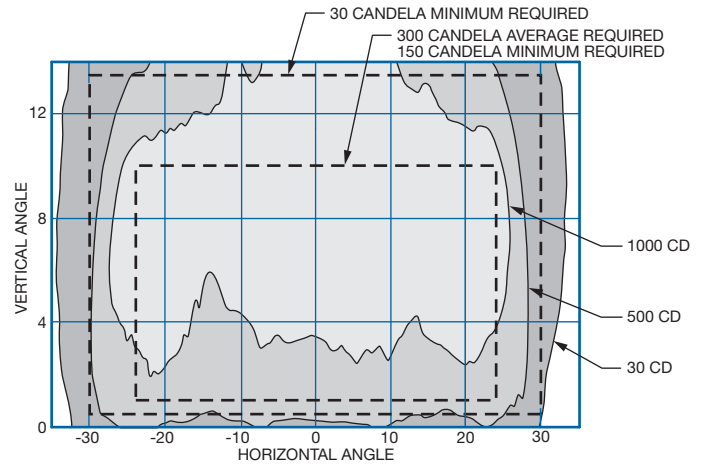
L-852S Stop Bar Light-Red
