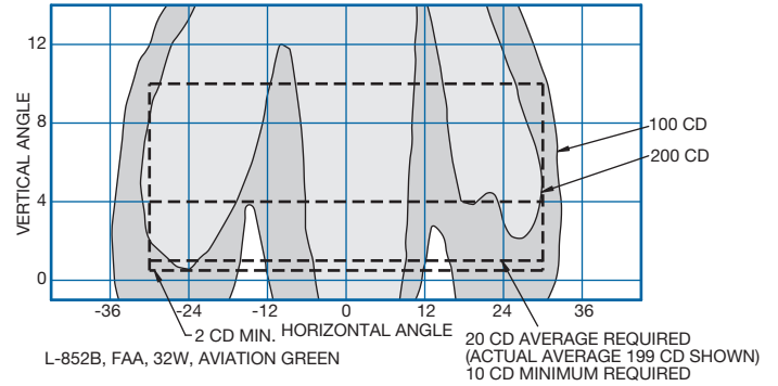
FAA L-852B Wide (Curved Section), CAT II
