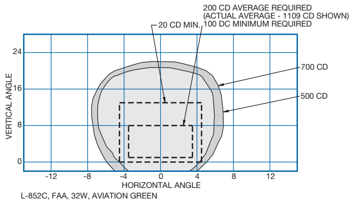
FAA L-852C Narrow (Straight Section), CAT III
