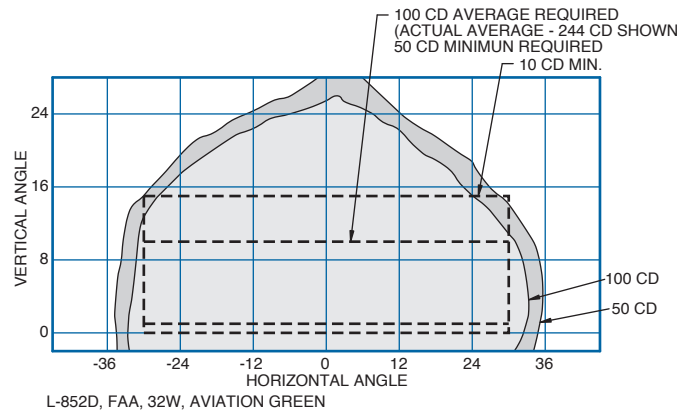
FAA L-852D Wide (Curved Section), CAT III
