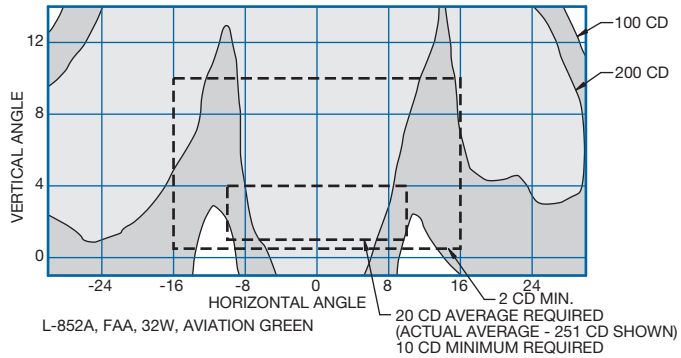
FAA L-852A Narrow (Straight Section), CAT II
