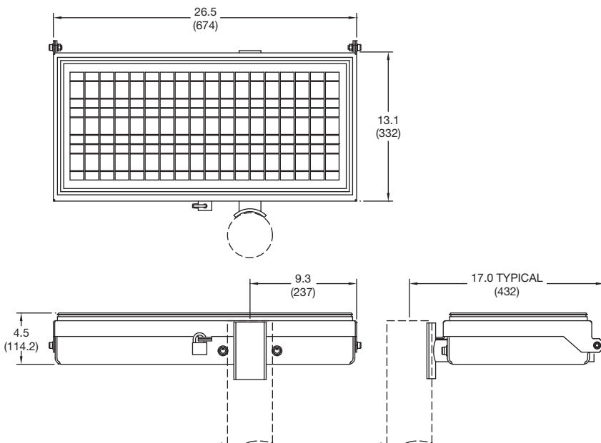
Shown with post side mount AV-SIGN-20-PM
