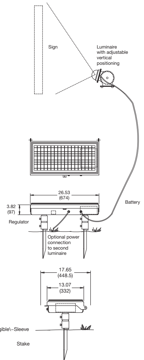
Shown with frangible stake mount (standard) AV-SIGN-20-FM
