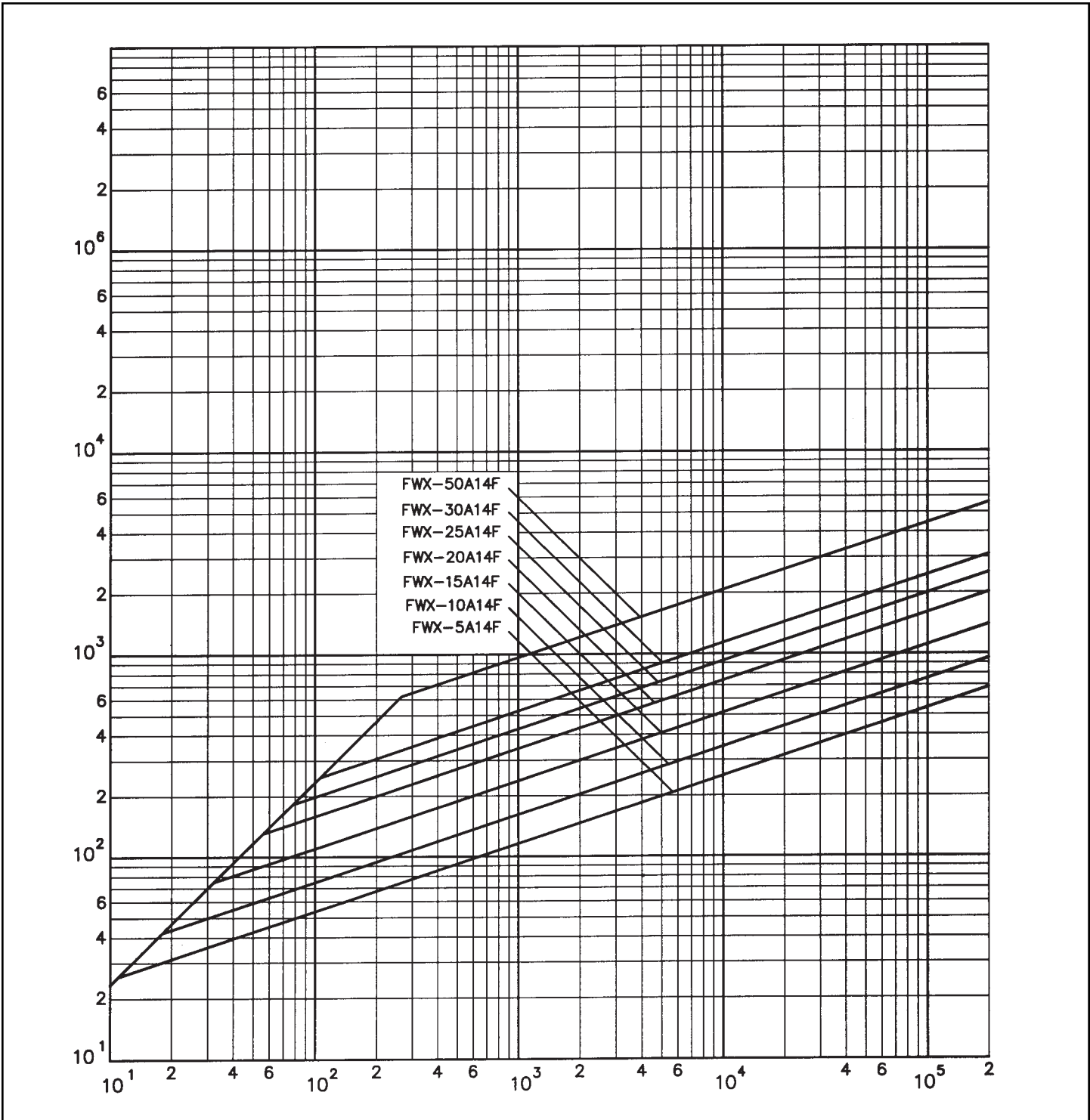
Peak Let-Through Cut-Off Current Characteristic Curves FWX 1A14F-30A14F
