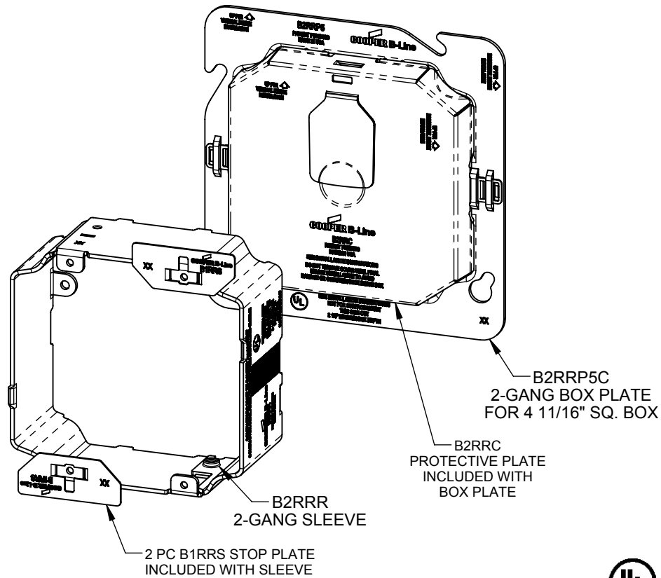
SLEEVE OPENING
