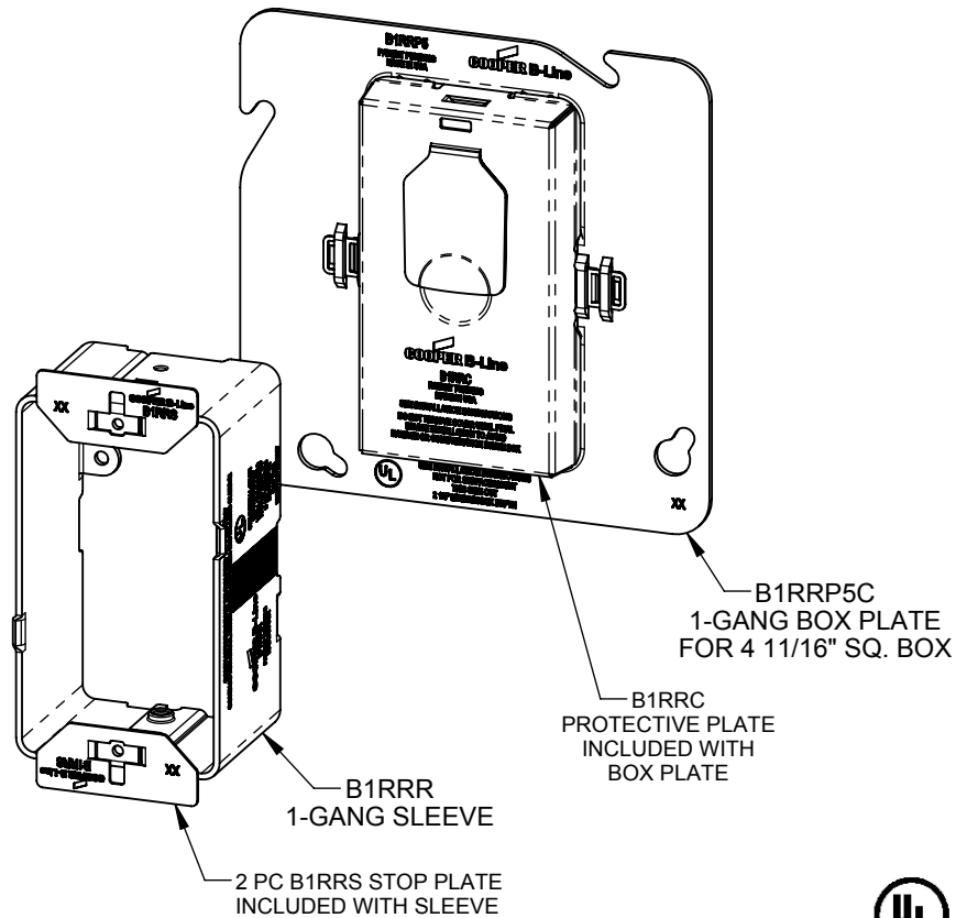
SLEEVE OPENING
