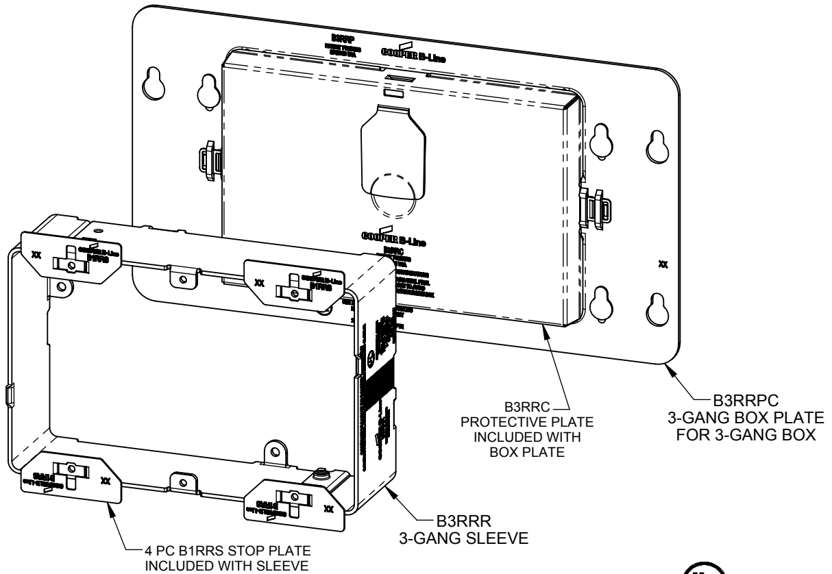
SLEEVE OPENING
