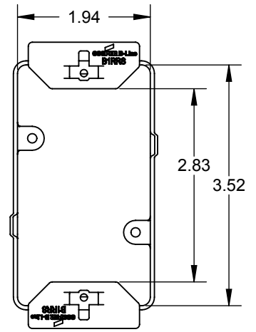
SLEEVE OPENING
