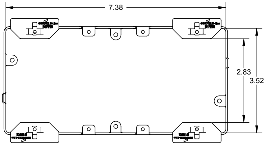
SLEEVE OPENING
