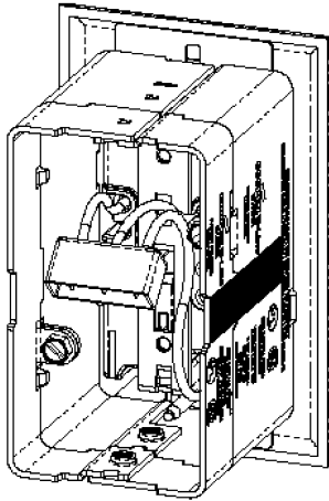
SLEEVE ASSEMBLY WITH SLEEVE EXTENDER
