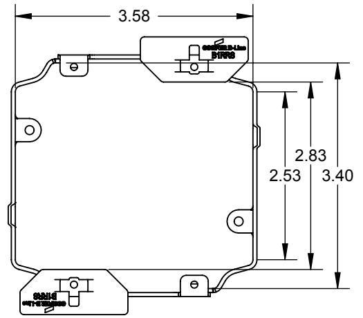
SLEEVE OPENING
