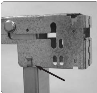
Locked in inner position.
