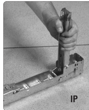
Step 2. Slide and lock legs into position. Inner position (IP) for clearance between pedestals or outer position (OP) for stacking.
