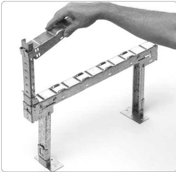
Step 3. Slide shelf bracket over vertical support. Pivot down to lock into correct height.
