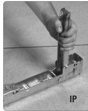
Step 2. Slide and lock legs into position. Inner position (IP) for clearance between pedestals or outer position (OP) for stacking.
