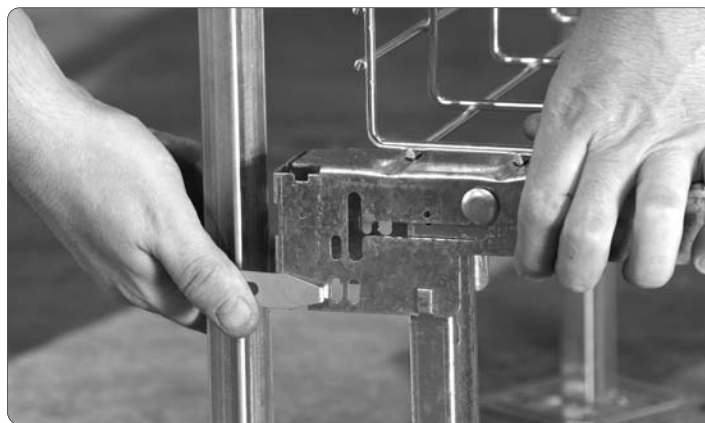
Step 5 (Optional). If desired, install pedestal clips.
