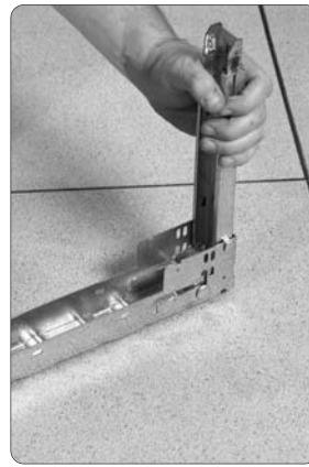
Step 2. Assemble stands with legs in outer position and adjust height.
