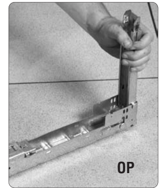
Step 2. Slide and lock legs into position. Inner position (IP) for clearance between pedestals or outer position (OP) for stacking.
