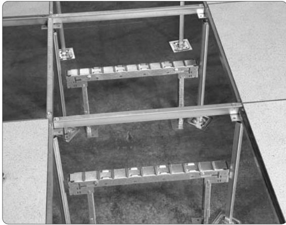
Step 1. Install first tier of stands.
