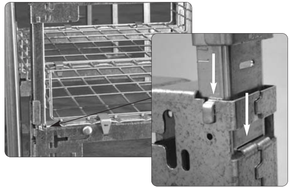
Step 4. Make sure tabs on bottom of legs are fully inserted into notches on the stand.
