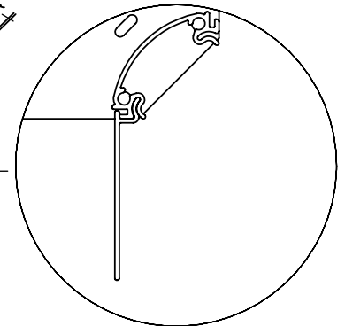
Detail top view: Splice fully engaged in corner post
