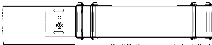
KwikSplice correctly installed
