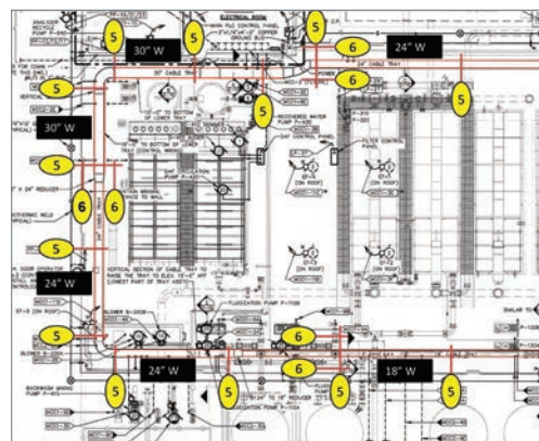
Cable tray layout with seismic bracing locations
