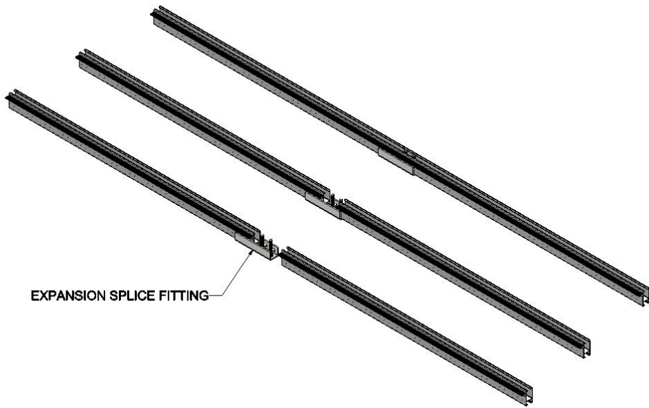
Landscape Rail with B172ESPLPA expansion splice clevis
